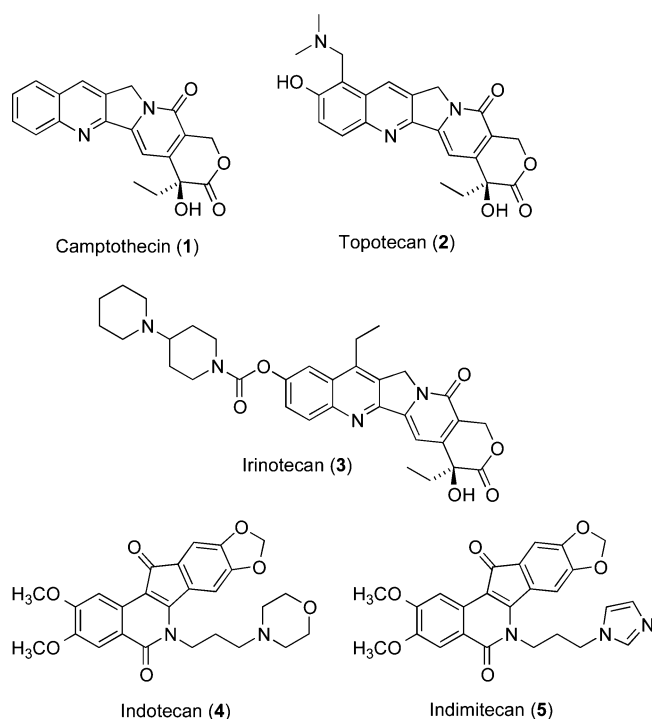
Figure 1. Representative Top1 inhibitors.
